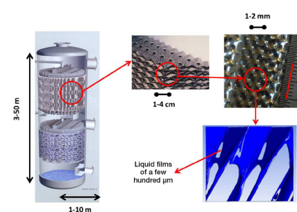
Multiscale problem of structured packings.
