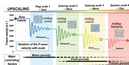
Principal P-wave velocity control factors for various study scales (from plug to seismic) (1) .
